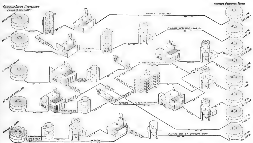
Fig. 2. How Pennsylvania Crude Oil Is Refined
